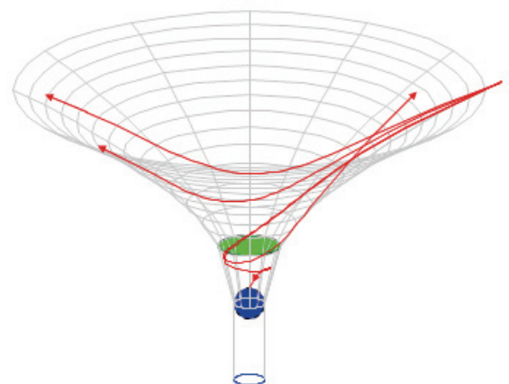
Fig. 22 Two-dimensional metaphor of the gravitational field, from the National Science Museum.
