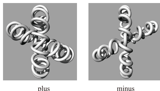
plus minus Fig. 8 Chirality between two Helical Tori
