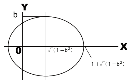
Fig. 23 Unit ellipse
