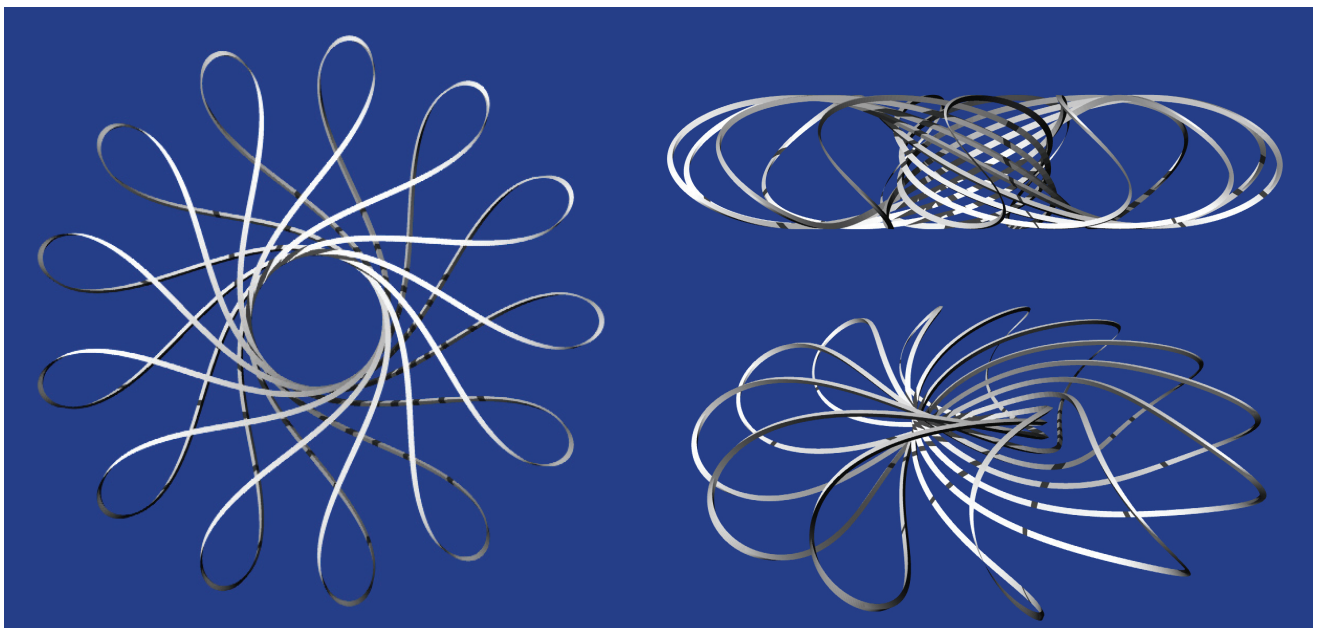
Fig.34 A Precessed Kepler Torus by chance
