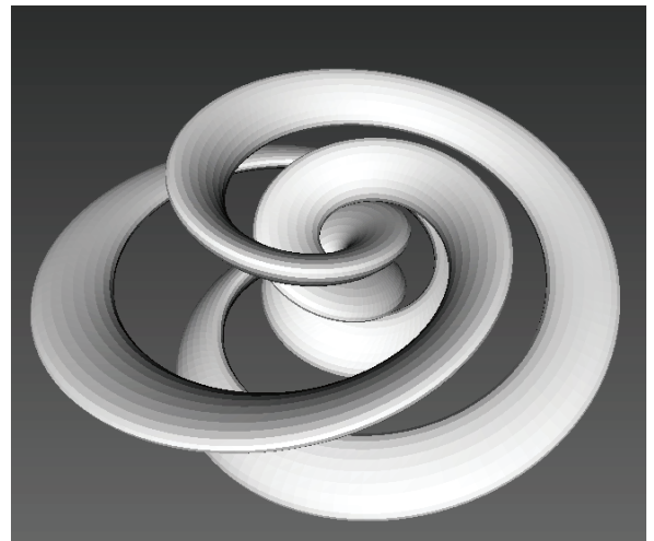
Fig. 21 Precessed elliptical orbit
