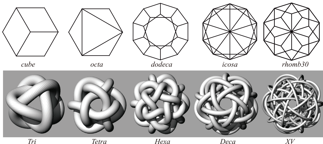
Fig. 7 Classification of the Poly-Twistor
