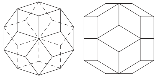
High-symmetry views
